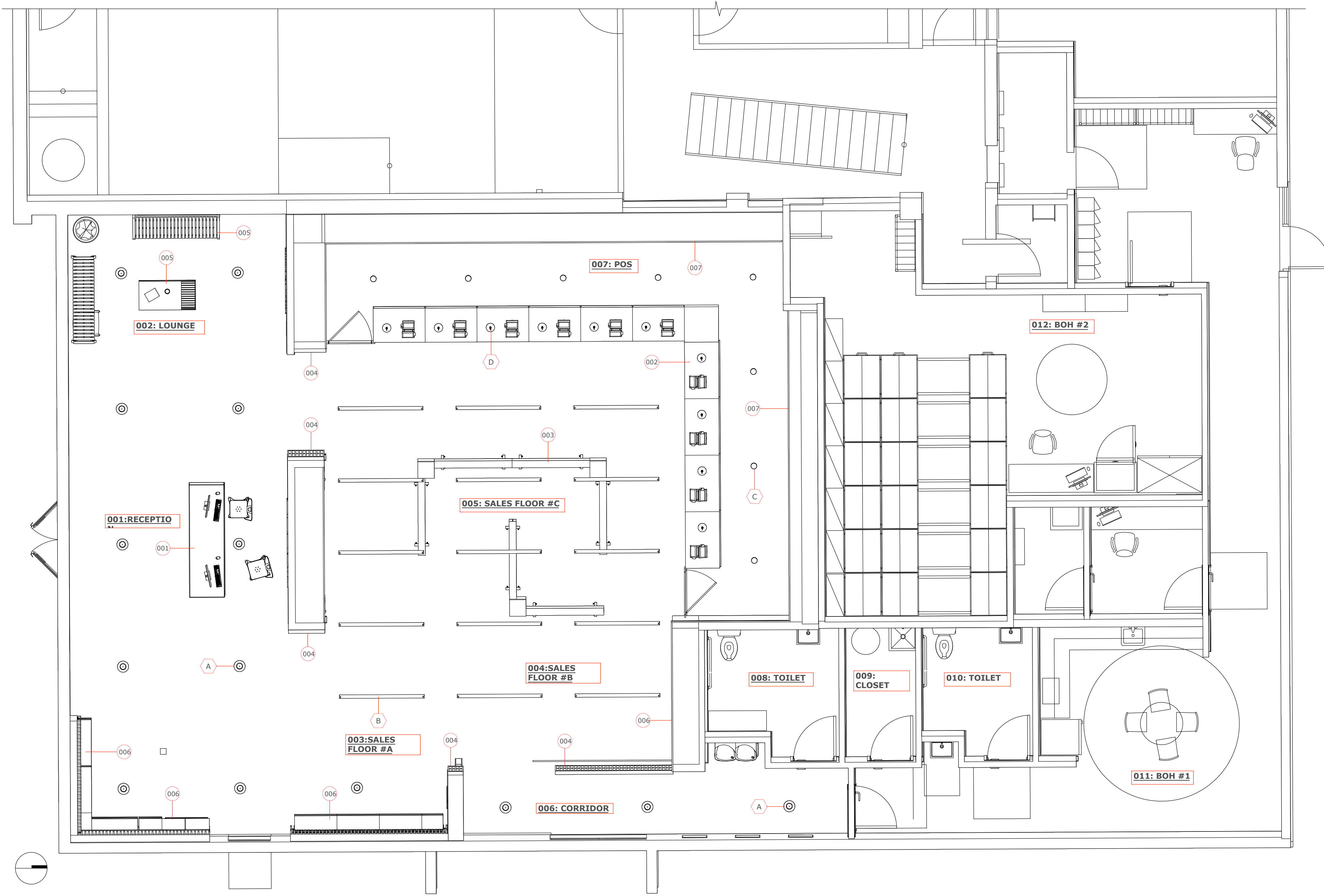
1 STORY - SALES FLOOR RCP Scale: 1/4" = 1'-0"
